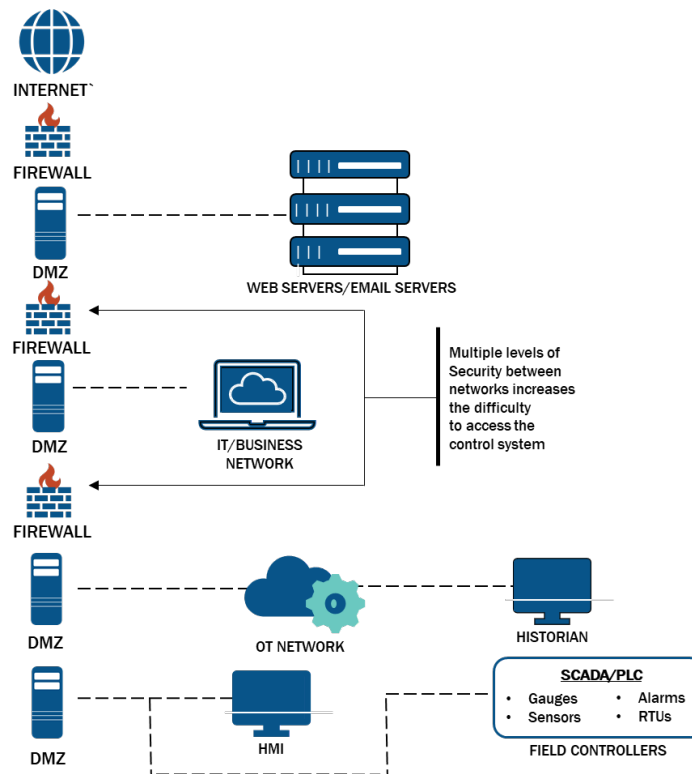
Figure 3: Network Segmentation
